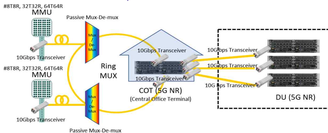
통신사업자 C 5G Optical Distributed Network
