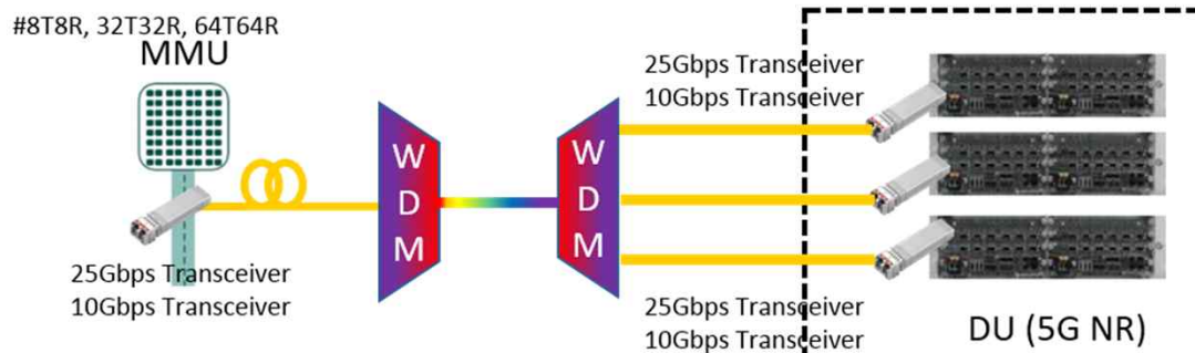
통신사업자 A,B 5G Optical Distributed Network
